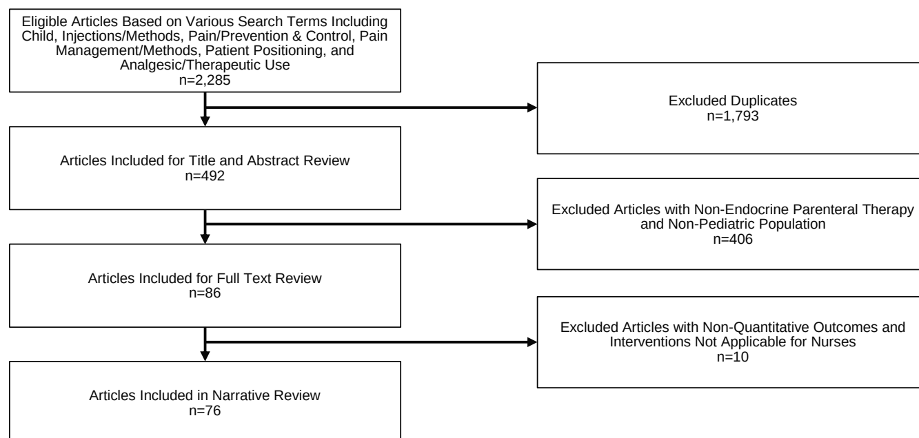
Supplementary Fig. (1). Article flow diagram.
